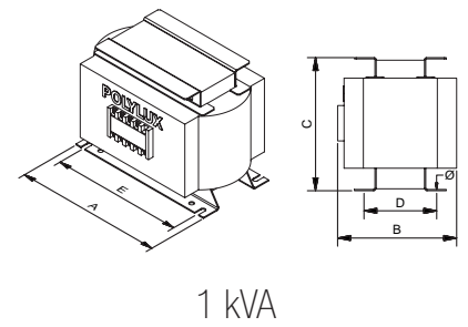
TH IP20
