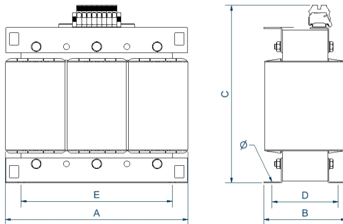
Dimensions (AxBxCxDxE): 480x290x480x184x400 mm 11Ø
