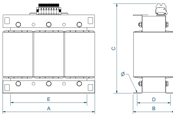
Dimensions (AxBxCxDxE): 480x310x480x204x400 mm 11Ø
