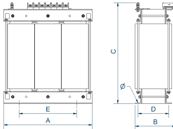
Dimensions (AxBxCxDxE): 670x280x615x170x426 mm 13Ø
