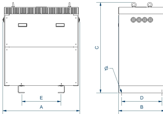
Dimensions (AxBxCxDxE): 1200x760x1555x672x690 mm 18∅
