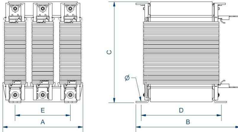
Dimensions (AxBxCxDxE): 150x140x185x85x100 mm 9Ø
