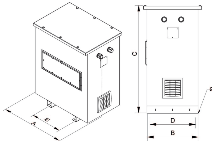
Dimensions (AxBxCxDxE): 745x413x735x370x350 mm 11Ø
