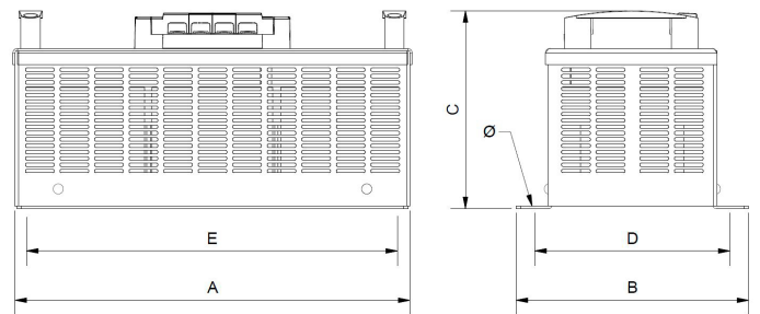
Dimensiones (AxBxCxDxE): 350x200x220x170x325 mm 6Ø
