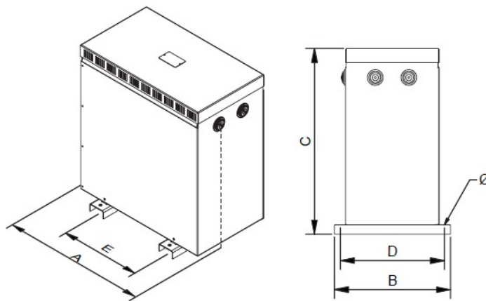
Dimensions (AxBxCxDxE): 528x418x644x375x345 mm 12Ø
