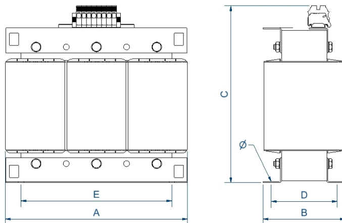
Dimensions (AxBxCxDxE): 360x270x353x202x300 mm 11Ø
