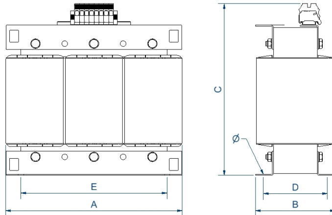
Dimensions (AxBxCxDxE): 360x240x353x172x300 mm 11Ø
