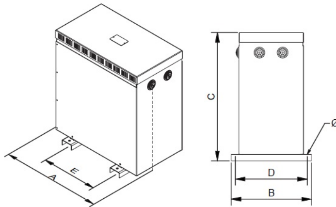
Dimensions (AxBxCxDxE): 970x670x1250x582x470 mm 18Ø
