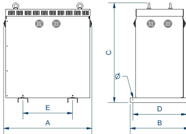
Dimensions (AxBxCxDxE): 597x415x710x375x350 mm 12Ø
