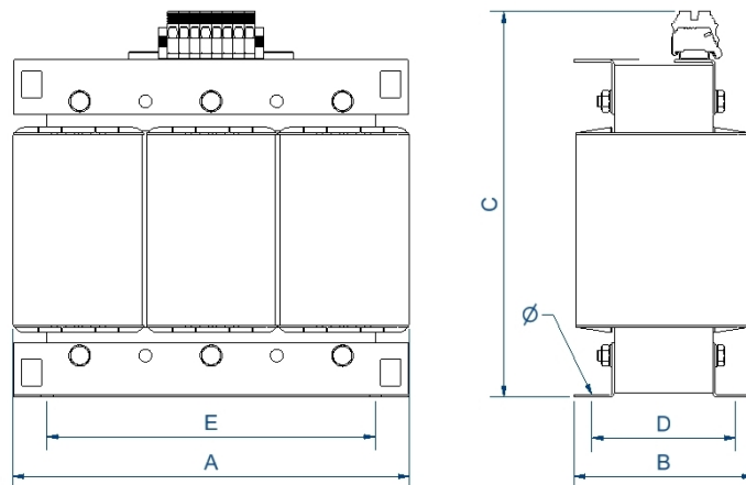
Dimensions (AxBxCxDxE): 300x134x303x125x250 mm 9Ø
