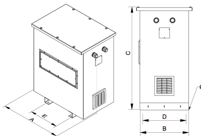
Dimensions (AxBxCxDxE): 970x621x1142x500x426 mm 12∅
