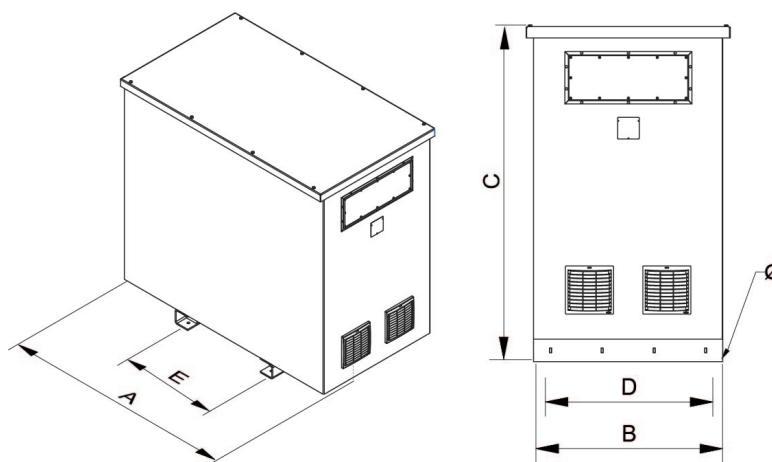
Dimensions (AxBxCxDxE): 1947x1093x1790x900x790 mm 20Ø
