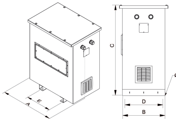
Dimensions (AxBxCxDxE): 1040x892x1366x714x485 mm 18Ø
