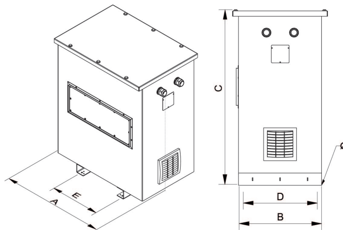
Dimensions (AxBxCxDxE): 970x621x1142x500x426 mm 12Ø
