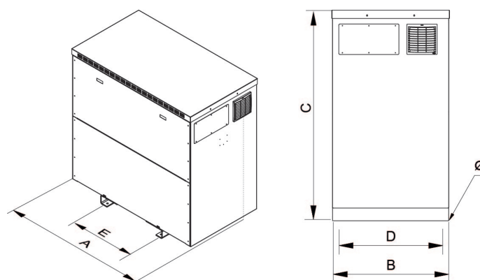
Dimensiones (AxBxCxDxE): 1820x1000x1800x900x790 mm 20Ø
