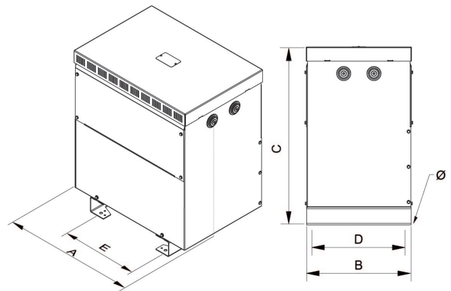
Dimensiones (AxBxCxDxE): 528x418x644x375x345 mm 12
