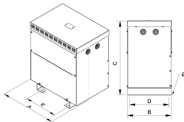
Dimensiones (AxBxCxDxE): 528x418x644x375x345 mm 12
