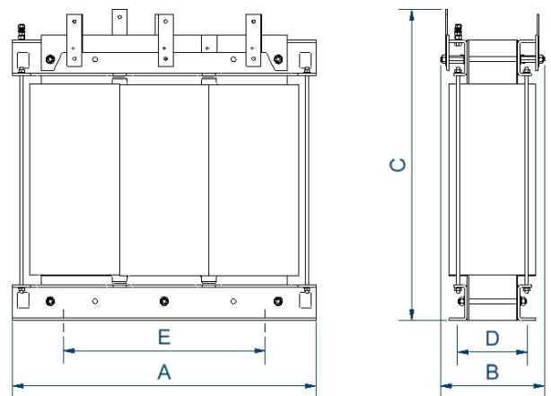
Dimensiones (AxBxCxDxE): 670x360x690x250x426 mm 13
