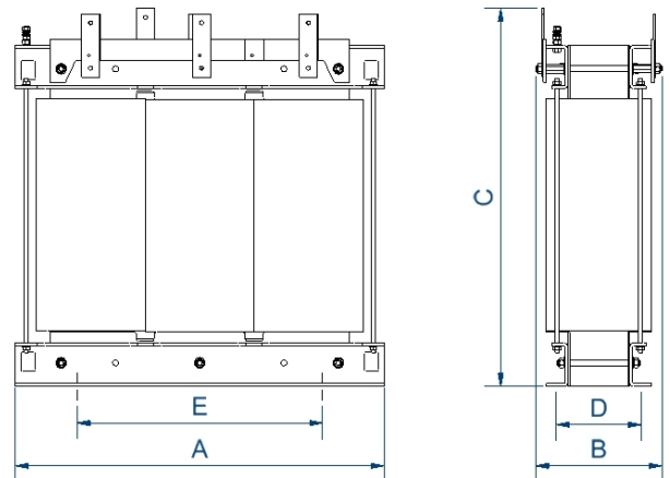
Dimensiones (AxBxCxDxE): 1070x550x1220x460x690 mm 17
