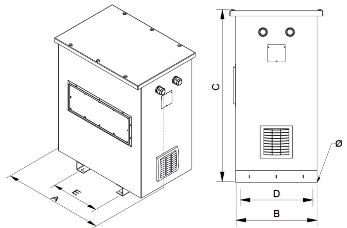
Dimensiones (AxBxCxDxE): 970x625x1150x500x426 mm 12Ø
