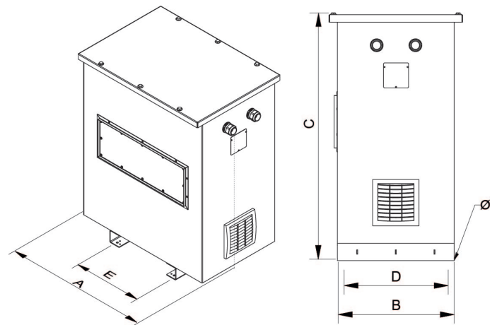
Dimensiones (AxBxCxDxE): 1550x1000x1750x806x684 mm 18Ø
