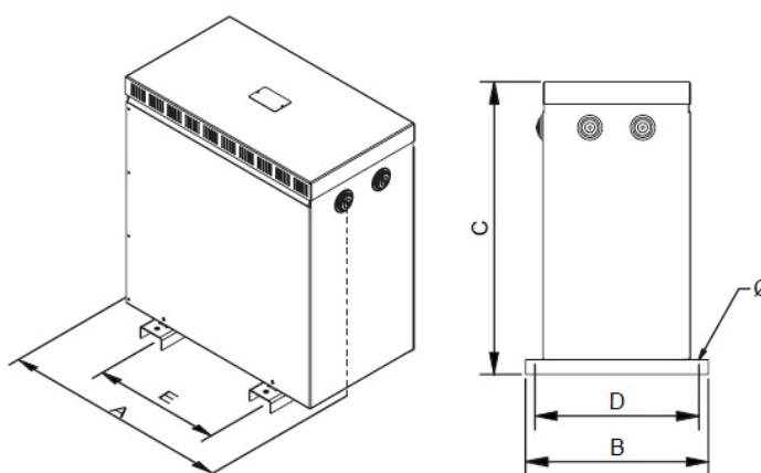
Dimensions (AxBxCxDxE): 240x190x250x180x150 mm 6Ø
