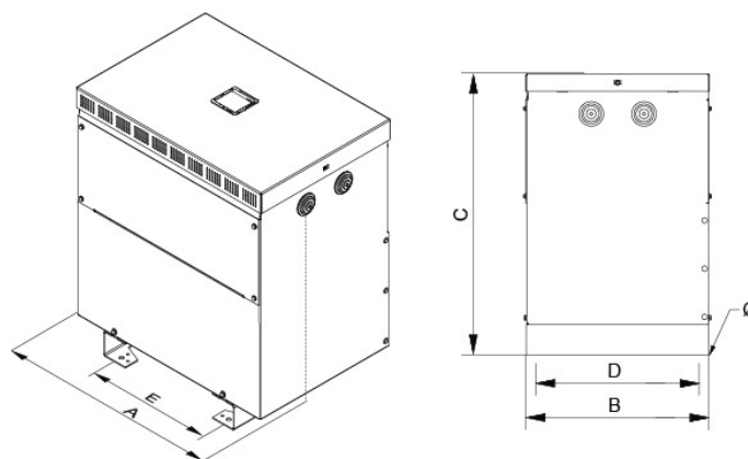
Dimensiones (Ax BxCxDxE): 480x340x500x300x300 mm 12Ø
