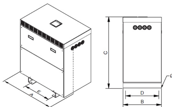
Dimensiones (Ax BxCxDxE): 1200x770x1555x672x690 mm 18Ø
