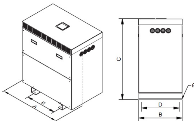
Dimensions (AxBxCxDxE): 1200x770x1555x672x690 mm 18Ø
