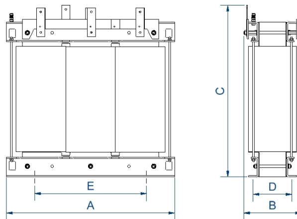
Dimensions (AxBxCxDxE): 1300x700x1365x600x800 mm 18Ø
