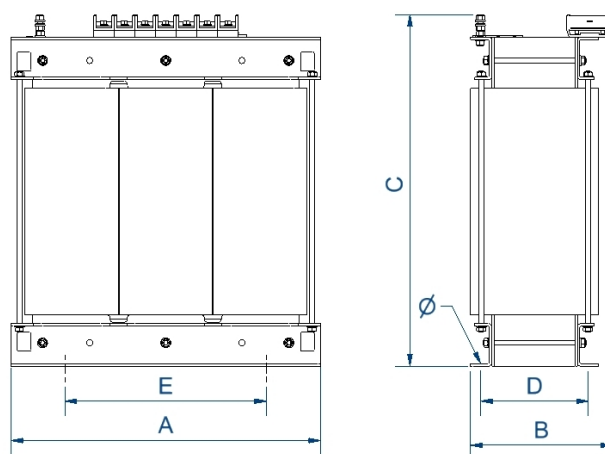
Dimensions (AxBxCxDxE): 640x325x500x179x426 mm 11Ø
