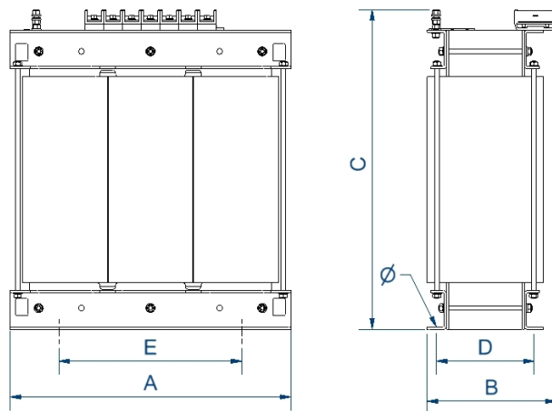
Dimensions (AxBxCxDxE): 640x400x537x199,5x426 mm 11Ø
