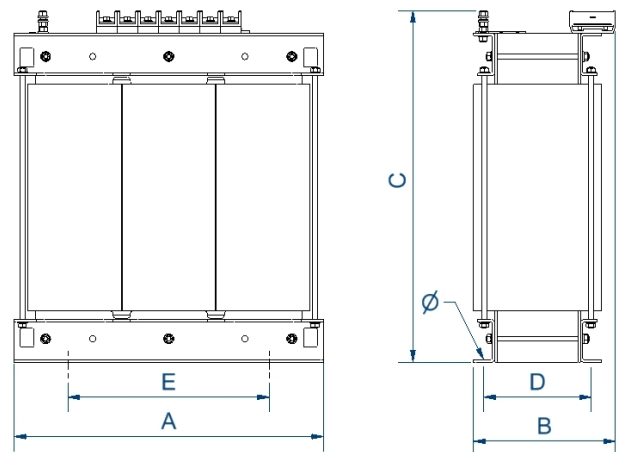
Dimensiones (AxBxCxDxE): 640x400x537x199,5x426 mm 11Ø
