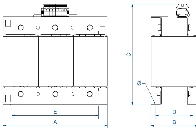
Dimensions (AxBxCxDxE): 360x144x372x122x300 mm 11Ø
