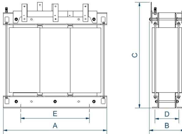
Dimensions (AxBxCxDxE): 714x450x692x209x426 mm 11Ø
