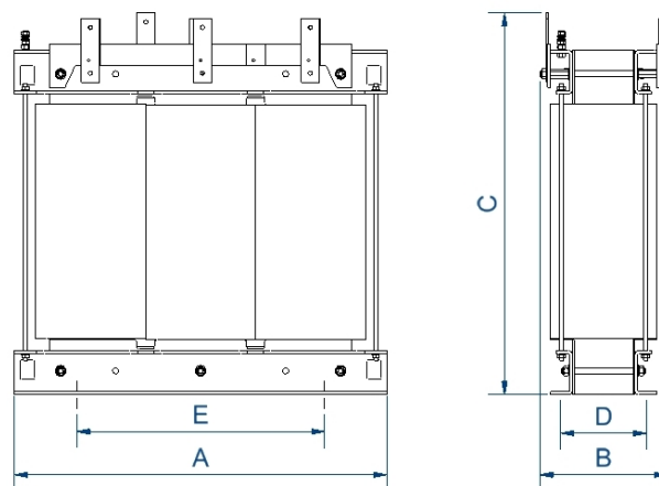
Dimensiones (AxBxCxDxE): 714x450x692x209x426 mm 11Ø
