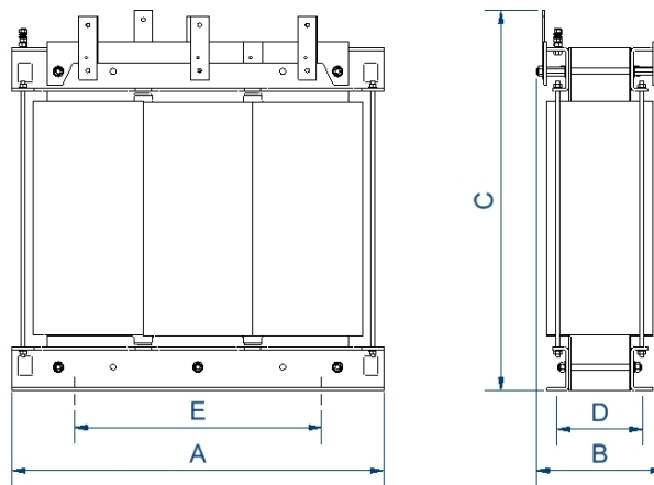
Dimensions (AxBxCxDxE): 1083x700x1200x600x690 mm 18Ø
