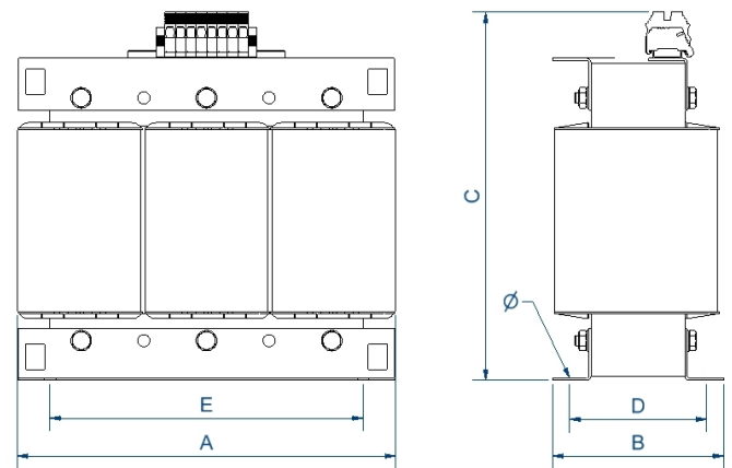
Dimensiones (AxBxCxDxE): 300x124x320x102x250 mm 9Ø
