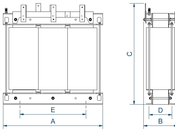
Dimensions (AxBxCxDxE): 1083x700x1265x600x690 mm 18Ø
