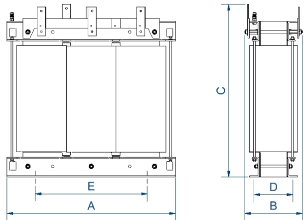
Dimensiones (AxBxCxDxE): 1083x700x1265x600x690 mm 18Ø
