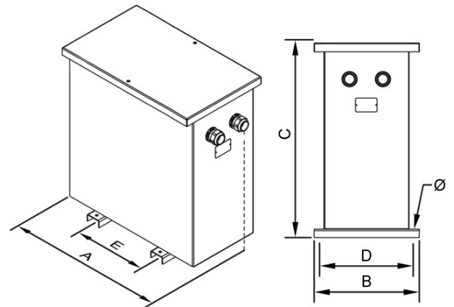
Dimensiones (AxBxCxDxE): 510x360x684x320x250 mm 11Ø
