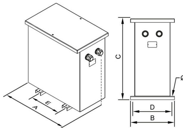
Dimensiones (AxBxCxDxE): 970x621x1142x500x426 mm 12Ø
