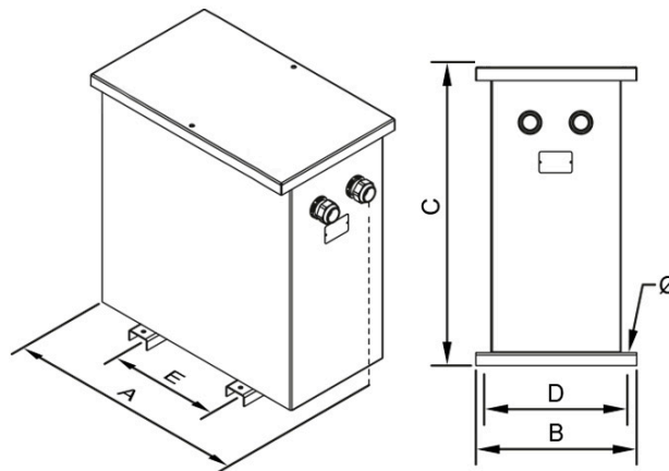
Dimensions (AxBxCxDxE): 1947x1093x1790x900x790 mm 20Ø
