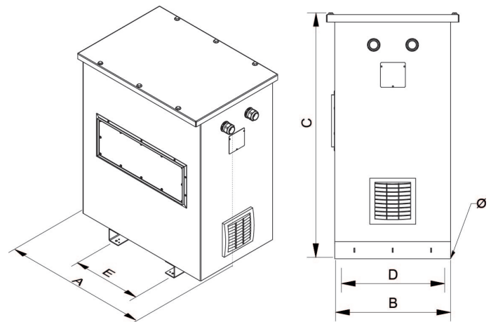
Dimensiones (AxBxCxDxE): 1550x1000x1746x806x684 mm 18Ø
