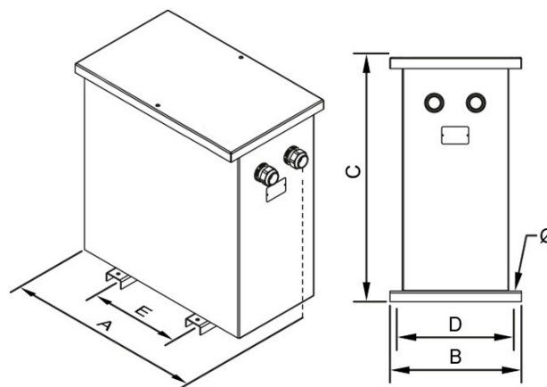
Dimensiones (AxBxCxDxE): 1550x1000x1746x806x684 mm 18Ø
