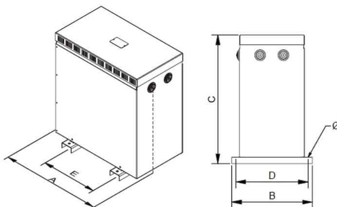
Dimensiones (AxBxCxDxE): 458x340x500x300x300 mm 12∅
