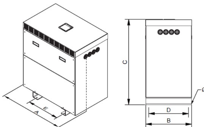
Dimensiones (AxBxCxDxE): 1200x760x1555x672x690 mm 18Ø
