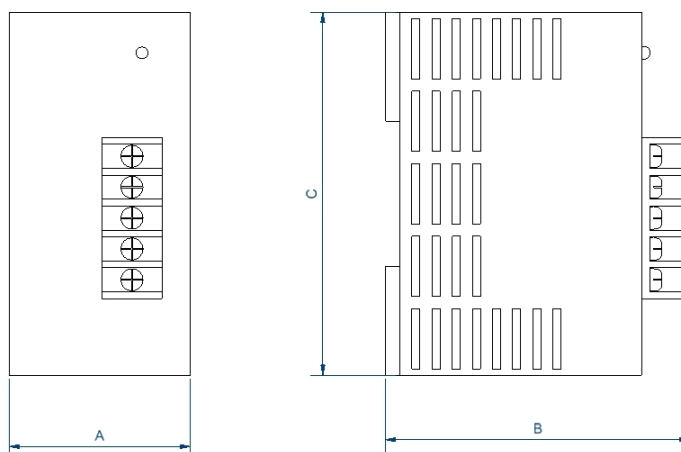
Dimensiones (AxBxCxDxE): 100x121x110 mm
