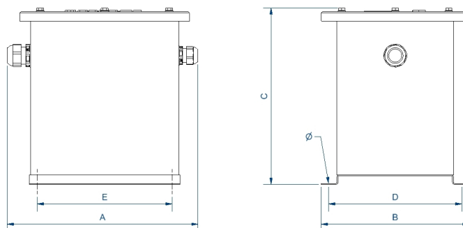
Dimensions (Ax BxCxDxE): 150x165x210x145x125 mm 7Ø
