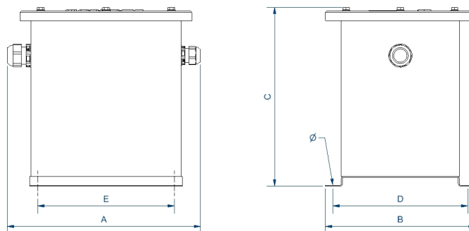
Dimensions (AxBxCxDxE): 195x198x220x178x173 mm 7Ø
